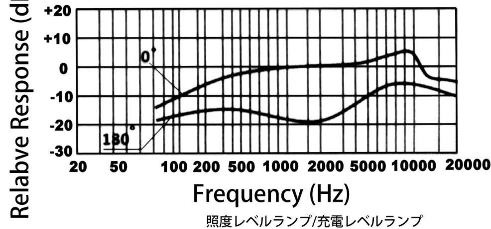
周波数応答グラフ (Frequency response graph)
